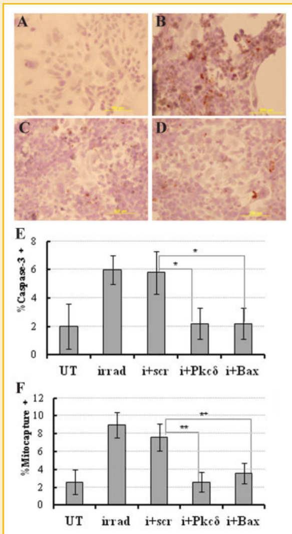
Fig. 4. Inhibition of pro-apoptotic Pkcδ or Bax protein expression decreases salivary gland cell sensitivity to radiation damage in vitro. (A) Non-irradiated control cells stained with caspase-3 antibody and hematoxylin show no caspase-3 activity. (B) Radiation treatment alone significantly increases caspase-3 activity in salivary gland monolayer cultures (caspase-3 positive cells are dark brown on hematoxylin counterstain). Pre-treatment with (C) nanoparticle/ Pkcδ siRNA complexes or (D) nanoparticle/ Bax siRNA complexes reduces caspase-3 staining in irradiated salivary gland cells compared to non-treated cells. (E) Quantitative analysis of the caspase-3 staining based on cell counts within a defined region of the microscopic field. Percentage of caspase-3 positive cells is derived from number of caspase-3 positive cells/total number of cells counted. UT, untreated control cells; irrad, irradiated cells; i+scr, irradiated cells pretreated with scrambled siRNA; i+ Pkcδ or Bax , irradiated cells pretreated with siRNA to Pkcδ or Bax ( n = 5 , *P < 0.05 ). (F) Mitochondrial membrane disruption was determined using a Mitocapture assay 24 h after irradiation ( n = 5 randomly chosen microscopic fields of each sample group). Percentage of mitocapture-positive cells is derived from number of mitocapture positive cells/total number cells counted. UT, untreated cells; irrad, irradiated cells; i+scr, irradiated scrambled-siRNA treated cells; i+ Pkcδ , irradiated Pkcδ -siRNA treated cells; i+ Bax , irradiated Bax -siRNA treated cells. **P < 0.001 . Statistical significance was tested by ANOVA and Tukey's multiple comparison tests. [Color figure can be seen in the online version of this article, available at http://wileyonlinelibrary.com/journal/jcb ]
