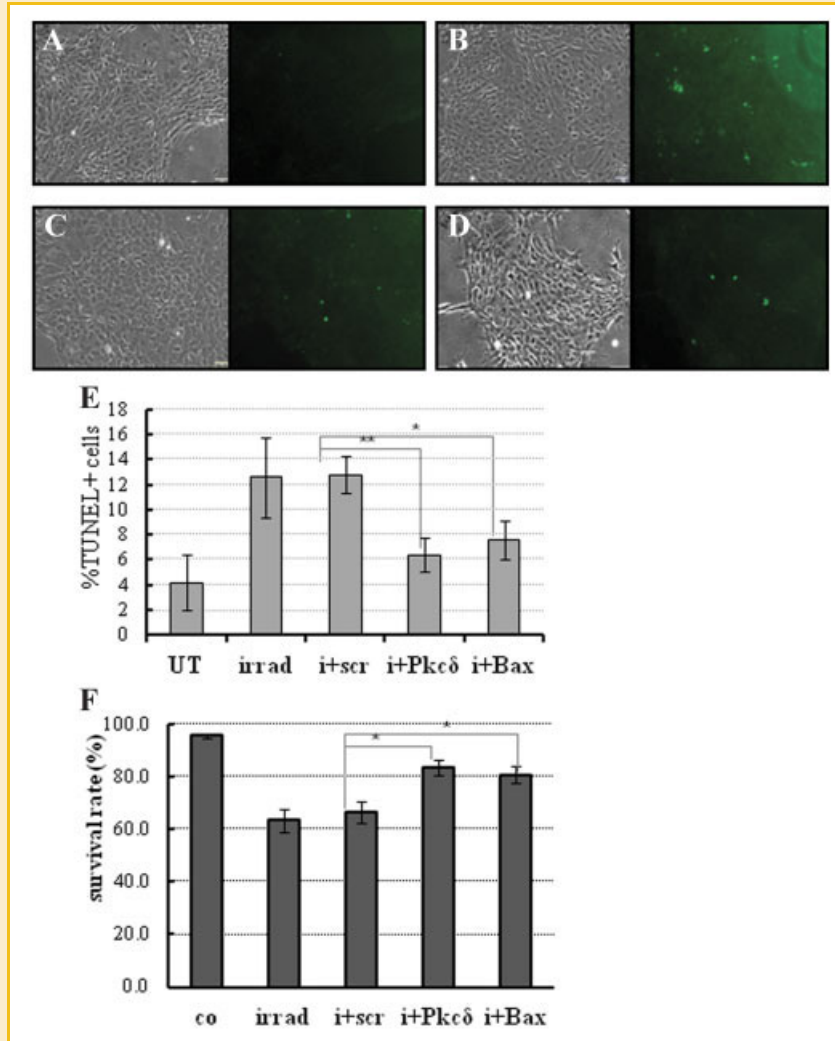
Fig. 5. siRNA knock down of Pkcδ or Bax expression reduces apoptotic cell death and increases radioprotection in irradiated primary salivary gland cells in vitro. (A–D) Identical bright-field and fluorescent images of cell monolayers after TUNEL staining to detect apoptotic cells (green). (A) Untreated cells have no detectable TUNEL-positive cells. (B) Treatment with 7.5 Gy radiation induces a significant increase in the number of apoptotic cells after 24 h. (C) Pretreatment with nanoparticle/ Pkcδ siRNA complexes before radiation treatment decreases the number of apoptotic cells. (D) Pretreatment with nanoparticle/ Bax siRNA complexes before radiation treatment also decreases the number of apoptotic cells. (E) Quantitative summary of TUNEL positive cells in control and siRNA-treated monolayers. Percentages represent TUNEL positive cells/total cells counted per microscopic field. Overall cell numbers were determined using parallel phase contrast images. UT, untreated control cells; irrad, irradiated cells; i+scr, irradiated cells pretreated with scrambled siRNA; i+ Pkcδ or Bax , irradiated cells pretreated with siRNA to Pkcδ or Bax . (F) Trypan blue staining confirms that the percentage of surviving cells was increased following pro-apoptotic gene knock down. Irradiation (7.5 Gy) was performed 24 h after pretreatment with nanoparticles complexed to Pkcδ or Bax siRNA, and live cells were counted on the following day using the Trypan-blue exclusion assay. (n = 5, ** P < 0.001; Statistical significance was tested by ANOVA and Tukey's multiple comparison tests.) Co, untreated cells; irrad, irradiated cells; i+scr, irradiated scrambled-siRNA treated cells; i+ Pkcδ , irradiated Pkcδ -siRNA treated cells; i+ Bax , irradiated Bax -siRNA treated cells. [Color figure can be seen in the online version of this article, available at http://wileyonlinelibrary.com/journal/jcb ]
