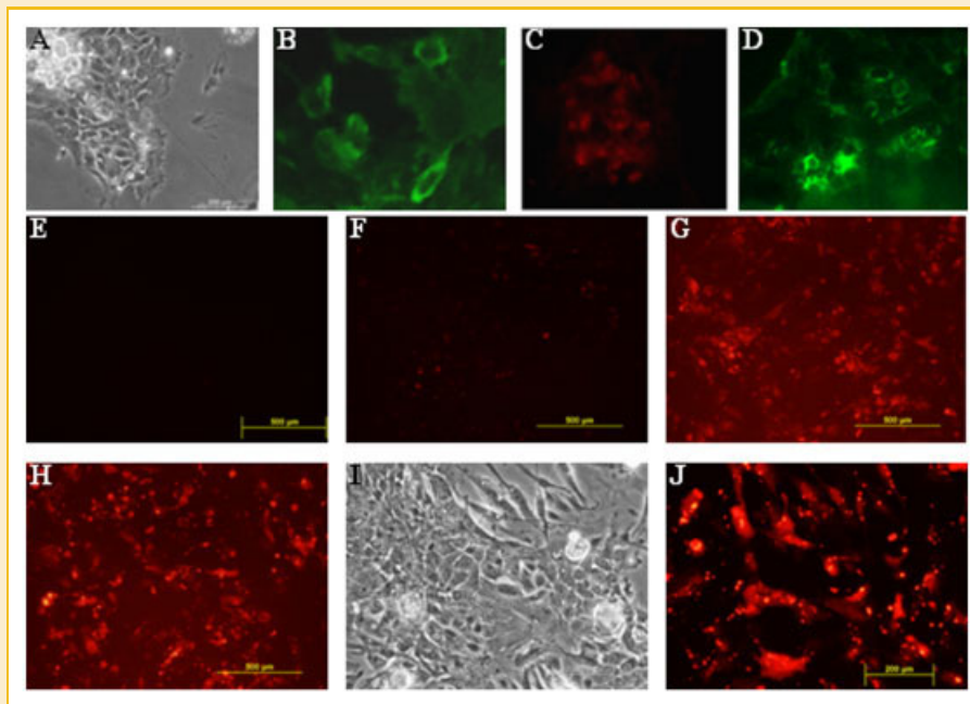
Fig. 1. Primary cell cultures derived from mouse submandibular gland include major cell types. (A) Phase contrast image of a monolayer culture. Representative photomicrographs of salivary gland specific lineage markers: (B) immunocytochemistry with antibody to \alpha -amylase detects secretory acinar cells (green); (C) immunocytochemistry with antibody to cytokeratin 19, a representative marker for differentiated duct cells (red); (D) immunocytochemistry with antibody to sca-1, a marker reported to label the progenitor cells of the salivary gland (green). (E) Cells treated with nanoparticles complexed to scrambled-siRNA show no fluorescence signal after transfection. (F) In no vector transfections, fluorescent Cy3-labeled siRNA is not internalized and serves as a negative control. (G) Lipofectamine-mediated delivery of Cy3-labeled siRNA (positive control) shows evenly distributed siRNA uptake after 8 h. (H) Nanoparticle-mediated Cy3-labeled siRNA shows similar level of distribution after 8 h. (I) Higher magnification phase contrast image and (J) fluorescent image of the same cells showing cellular internalization of siRNA mediated by the pH-responsive nanoparticles. [Color figure can be seen in the online version of this article, available at http://wileyonlinelibrary.com/journal/jcb ]
