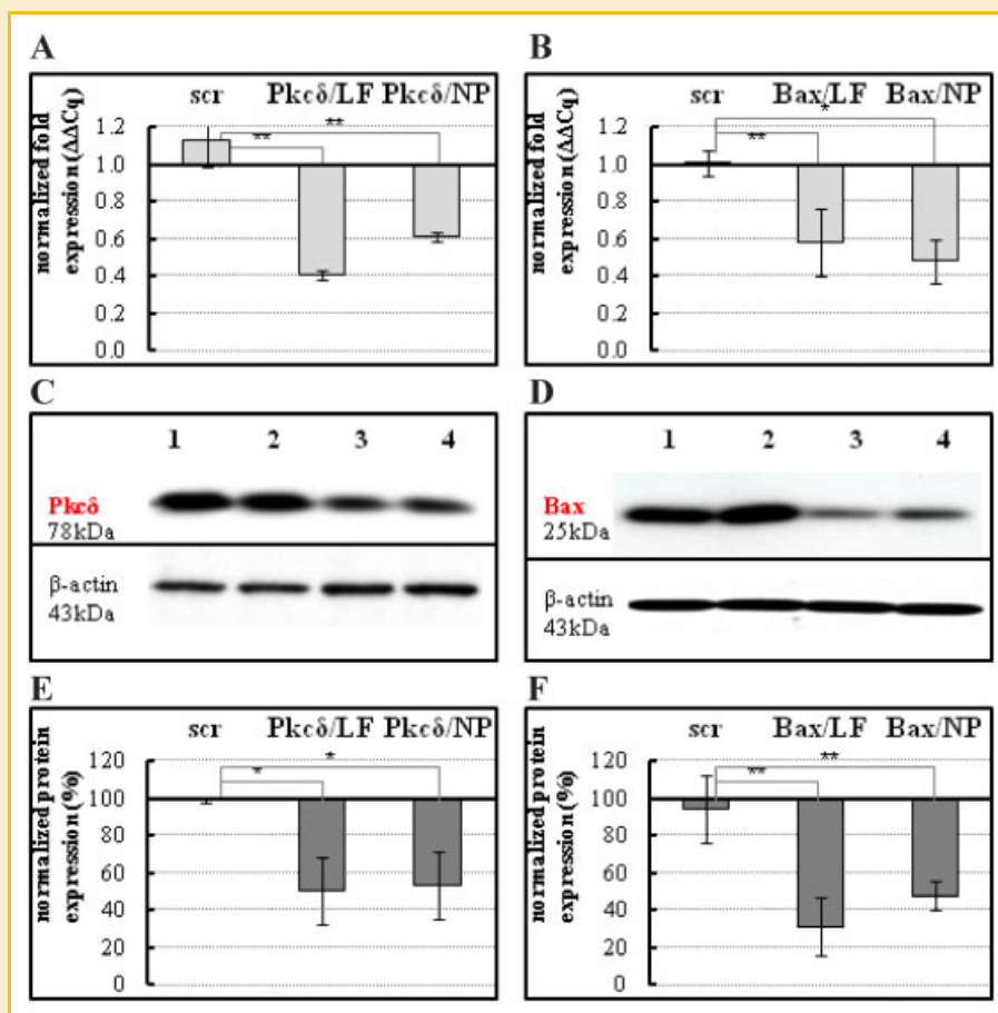
Fig. 2. siRNA knock down of Pkc \delta or Bax expression in cultured salivary gland cells. (A–B) mRNA expression was analyzed by qPCR 24 h following transfection. (A) Transfection with Pkc \delta siRNA using Lipofectamine (LF) or nanoparticles (NP) inhibits Pkc \delta mRNA expression compared to scrambled siRNA control (scr) delivered by nanoparticles; (B) Transfection with Bax siRNA using Lipofectamine (LF) or nanoparticles (NP) demonstrated efficient reduction of Bax mRNA expression levels. Results are representative of three replicates and compared to untreated controls (fold changes); * P < 0.05 by one-way analysis of variance with Dunnett's multiple comparison test. (C–D) The lysed cells were analyzed for expression levels of the two pro-apoptotic proteins on Western blots. (C) Pkc \delta , or (D) Bax protein expression was normalized to \beta -actin (blots were stripped and reprobed). Lane 1, untreated cells; lane 2, cells treated with scrambled siRNA control; lane 3, cells treated with Lipofectamine-mediated siRNA, as positive control; lane 4, cells treated with nanoparticle-mediated siRNA. (E–F) Graphs show quantification of protein band intensities from Western blot analysis, scanned by alpha imaging and measured using the ImageJ (NIH) software. LF, Lipofectamine; NP, nanoparticle complexes. Calculations were based on three measurements compared to untreated controls (protein level established as 100%); * P < 0.05 , ** P < 0.001 . [Color figure can be seen in the online version of this article, available at http://wileyonlinelibrary.com/journal/jcb ]
