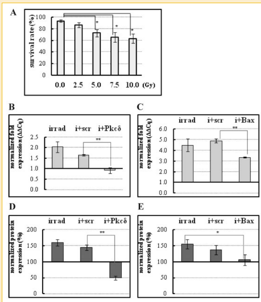
Fig. 3. siRNA knock down blocks radiation-induced increase of the pro-apoptotic genes Pkc \delta or Bax. (A) Dose response curve of irradiated salivary gland monolayer cultures. Cells were counted 48 h after the indicated dose of \gamma -ray radiation. 7.5 Gy single dose irradiation resulted in a significant ( P < 0.05 ), 40% reduction in cell survival, and was used in all subsequent experiments. Radiation normally increases Pkc \delta (B) or Bax (C) gene expression. However, nanoparticle-mediated siRNA knock down of Pkc \delta or Bax expression blocks the radiation-induced increase. Cells were irradiated 24 h after siRNA/nanoparticle addition, and mRNA levels were assayed by qPCR after an additional 24 h. Results are representative of three replicates and compared to the untreated controls. (D–E) Total protein extracts were analyzed by Western blot. Densitometric analysis of control and sample band ratios was conducted. The untreated control level of each protein was designated as 100%. (D) Radiation-induced Pkc \delta protein expression showed a statistically significant decrease in the presence of siRNA (i + Pkc \delta ) compared to the scrambled siRNA (scr) negative control. (E) Radiation-induced Bax protein level was also reduced in cells in the presence of siRNA/nanoparticle complexes (i + Bax) ( *P < 0.05 , **P < 0.001 , n = 3 ). Statistical significance was calculated using one-way analysis of variance with Tukey's multiple comparison tests.
